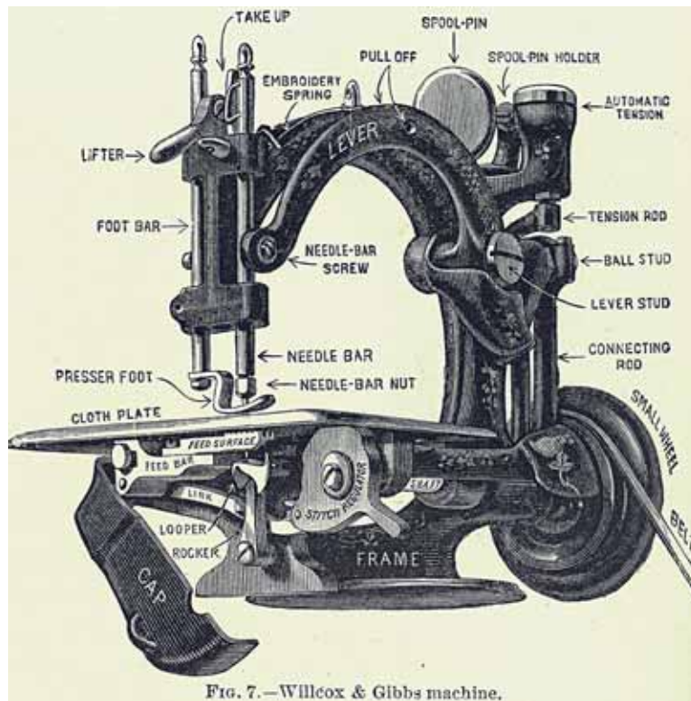
Fig. 7.—Willcox & Gibbs machine.
